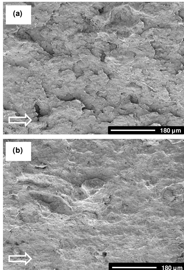
Figure 5. The surface morphology near (a) and away (b) from notch of 5 wt.% zeolit/HDPE
