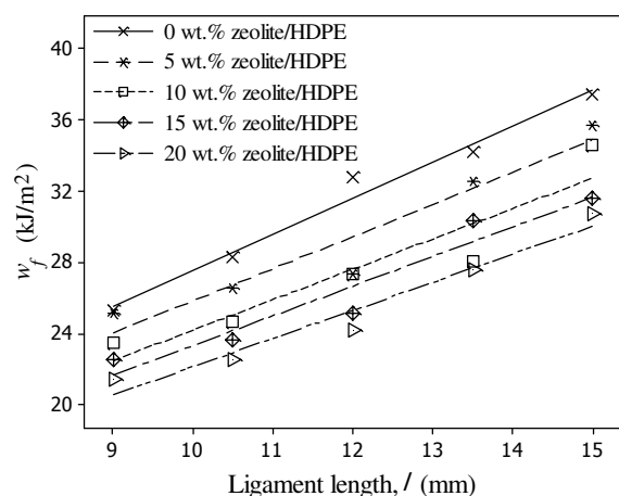
Figure 2. Specific total work of fracture plotted against ligament length for all specimens tested
