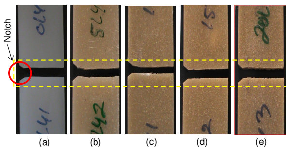
Figure 4. The SENB broken samples for (a) HDPE, (b) 5 wt.% zeolit/HDPE, (c) 10 wt.% zeolit/HDPE, (d) 15 wt.% zeolit/HDPE, and (e) 20 wt.% zeolit/HDPE
