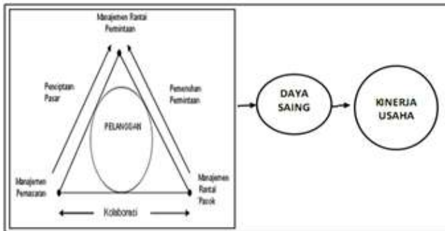
Figure 2: Theoretical Framwork
